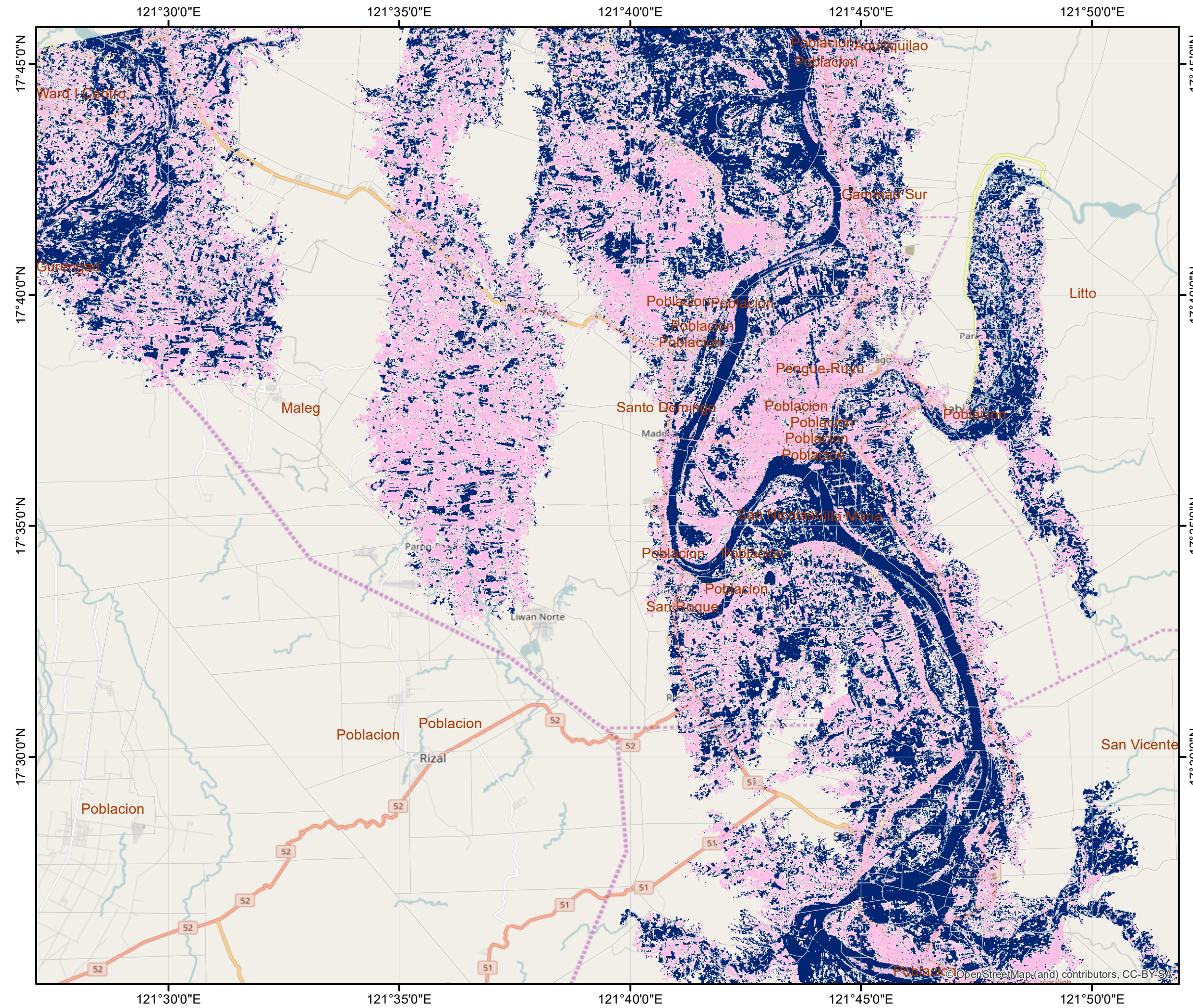
Map3: Typhoon HAIMA Flood in the Province of Cagayan, northern part of the Philippines observed on 27 October 2016
